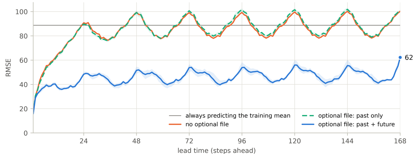
Validation RMSE at each lead time (line: mean over seeds, band: range over seeds)
